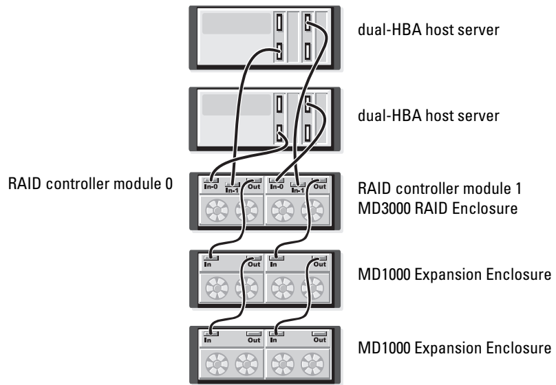
Figure 2-9. Cabling Two Hosts (With Dual-HBAs) Using Redundant Data Paths
