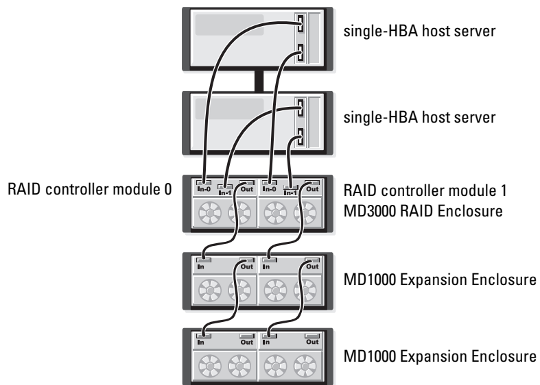
Figure 2-11. Cabling a Two-Node Cluster (Single HBA, Redundant Data Paths From Each Node)
