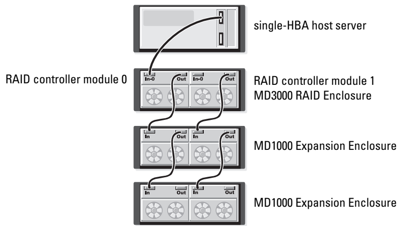
Figure 2-1. Cabling One Host With Nonredundant Data Paths
